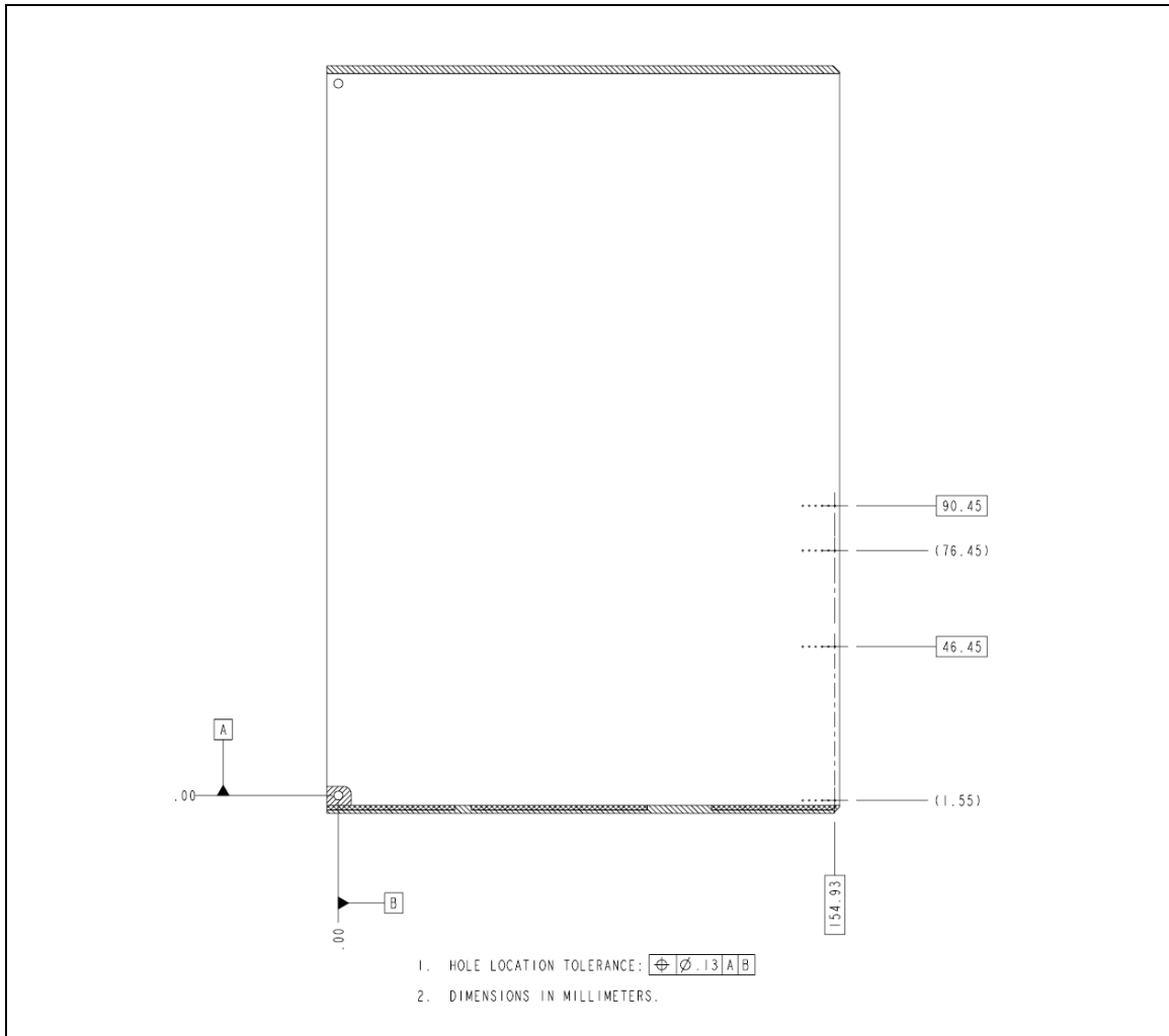
Figure A-4. eHM Physical Location on a 6U Peripheral Module
