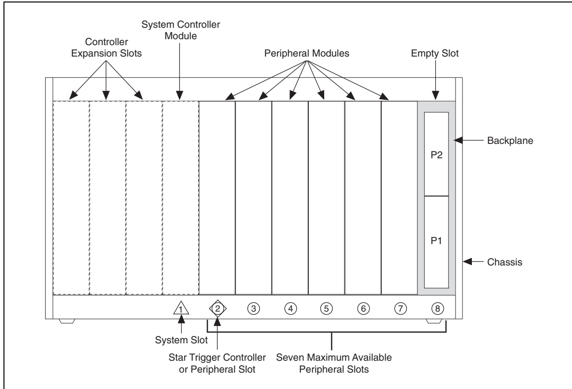
Figure 2-2. Example of a 33 MHz 3U PXI System (Single Bus Segment)
