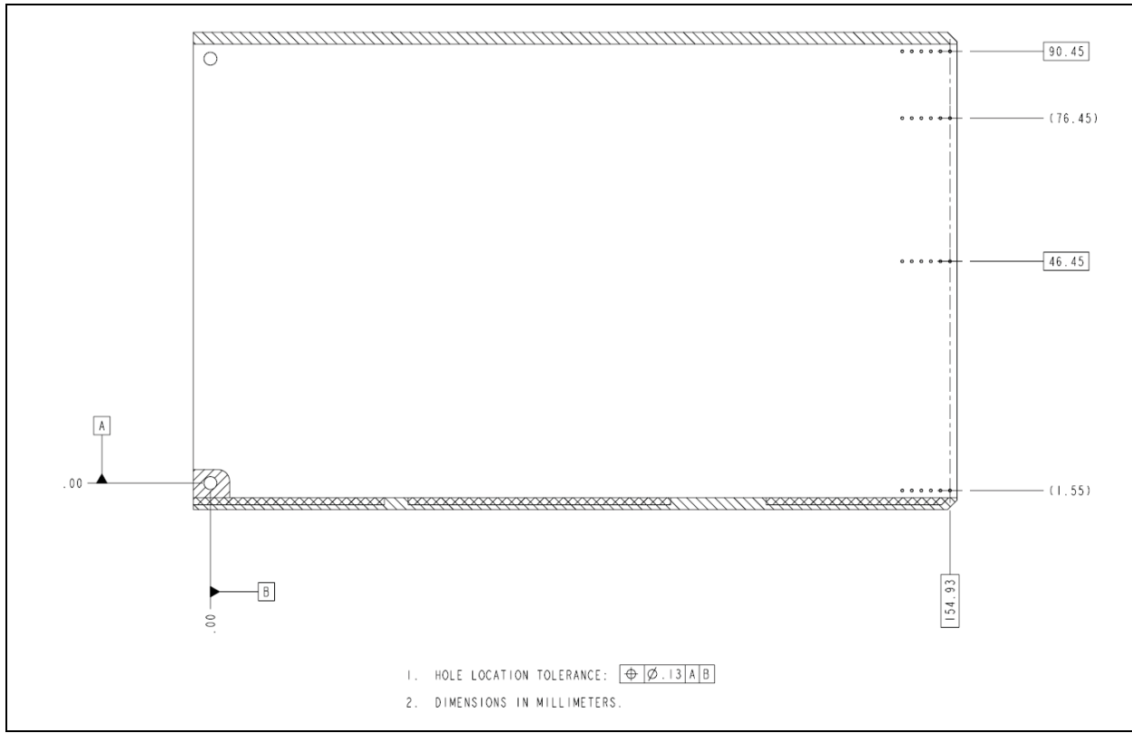
Figure A-3. eHM Physical Location on a 3U Peripheral Module
