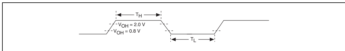
Figure 4-1. PXI Asynchronous Trigger Timing
