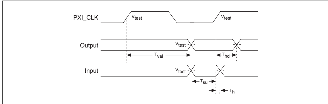
Figure 4-2. PXI Synchronous Trigger Timing
