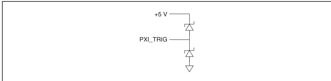
Figure 4-3. PXI Trigger Bus Termination
