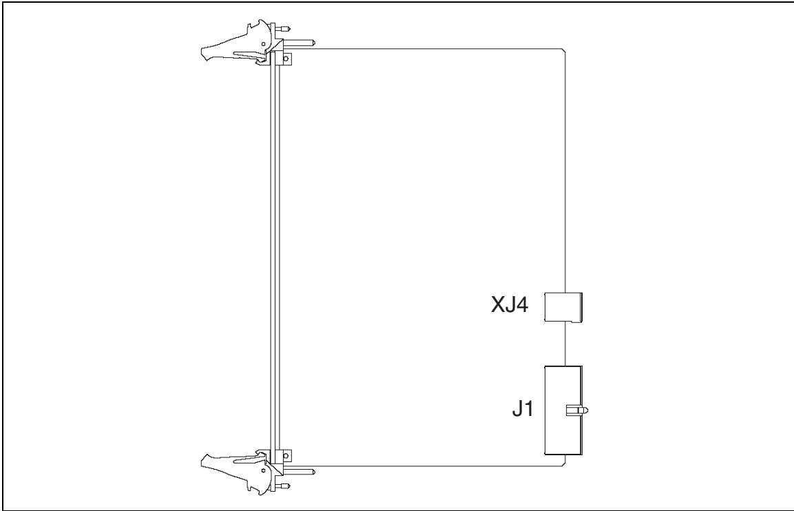
Figure A-2. 6U Hybrid Slot-Compatible PXI-1 Peripheral Module
