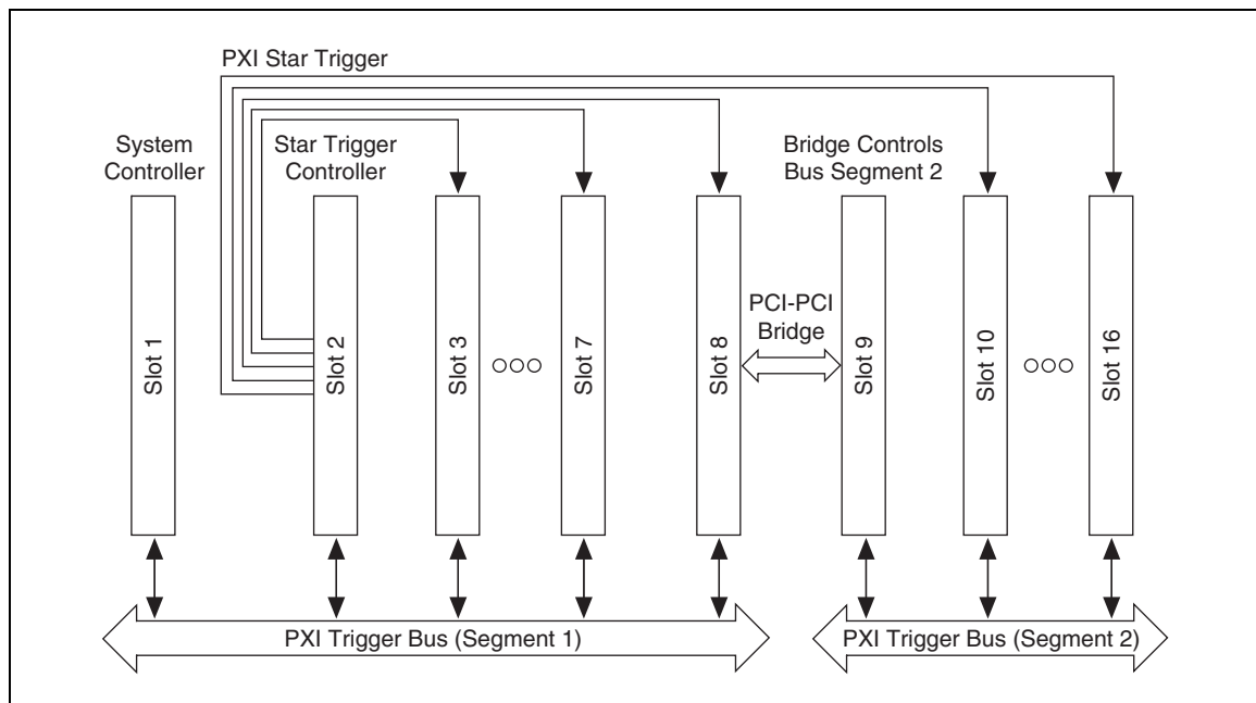
Figure 2-6. PXI Trigger Architecture for Two Bus Segments
